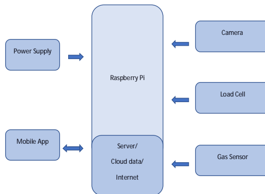
Fig.4. Block diagram
