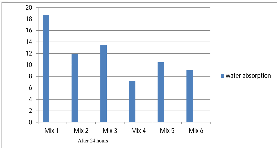
Fig.3 Water absorption test values for different trial mix
