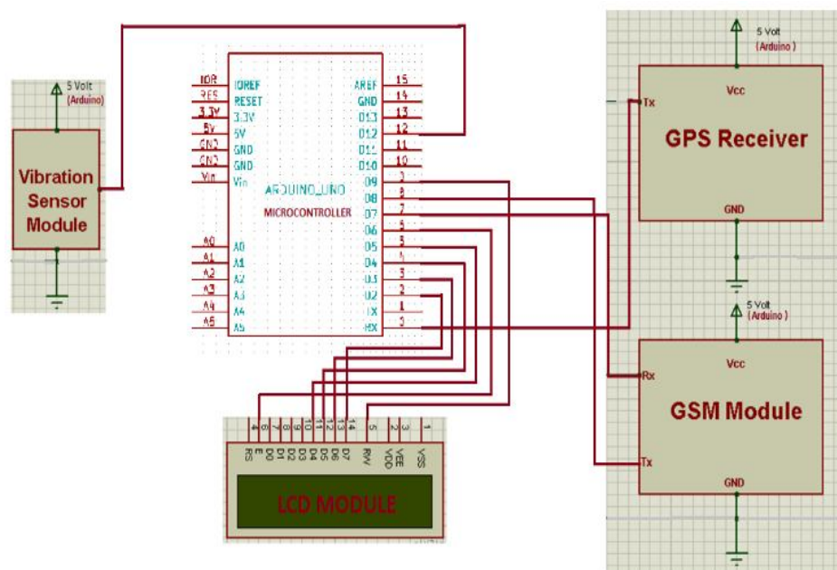
Fig. 1.Circuit diagram
