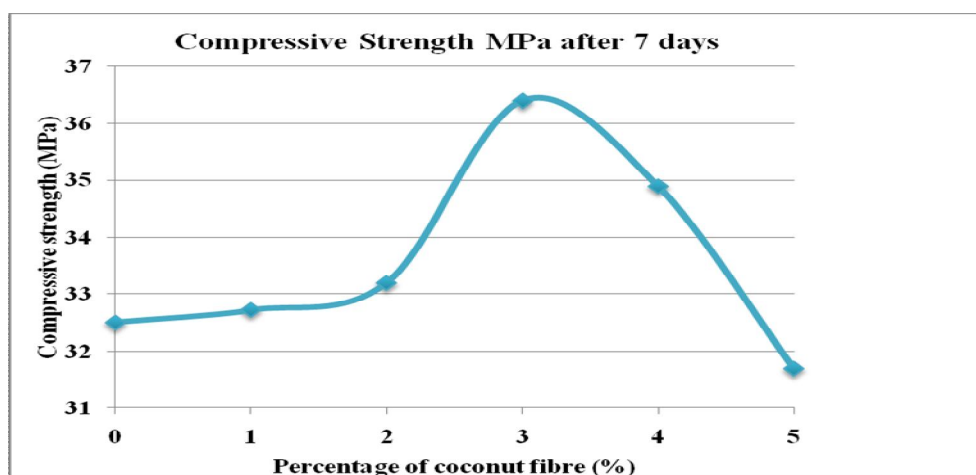
Fig 2: Compressive strength of coconut fibre reinforced concrete after 7 days of curing
