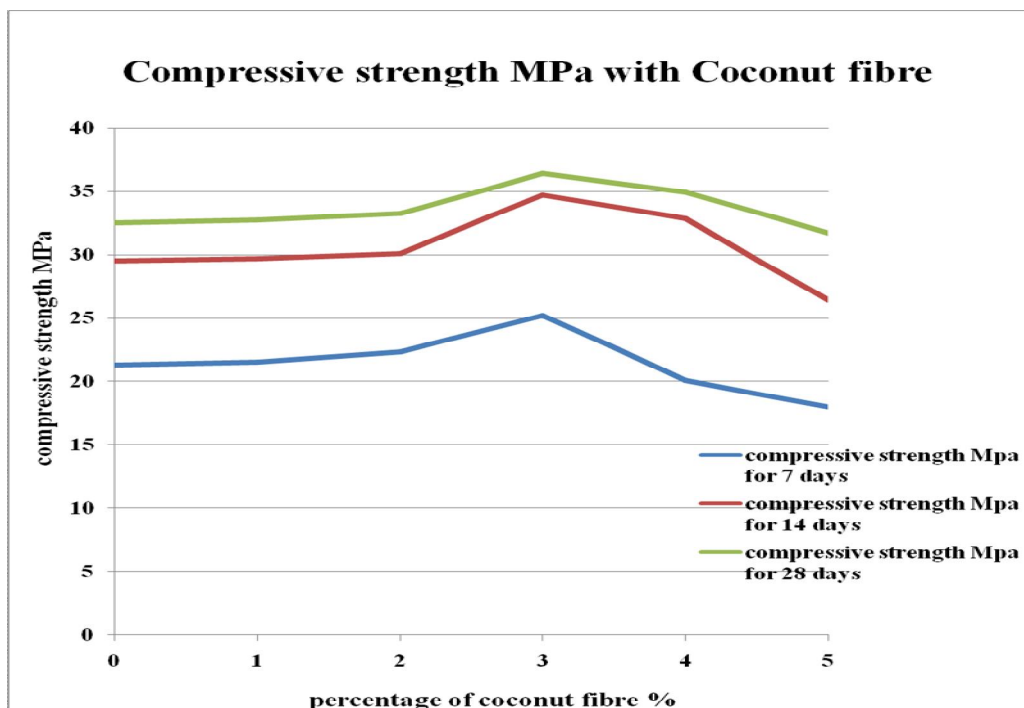
Fig 5: Comparative study on compressive strength of coconut fibre reinforced concrete after 7 days, 14 days and 28 days of curing
