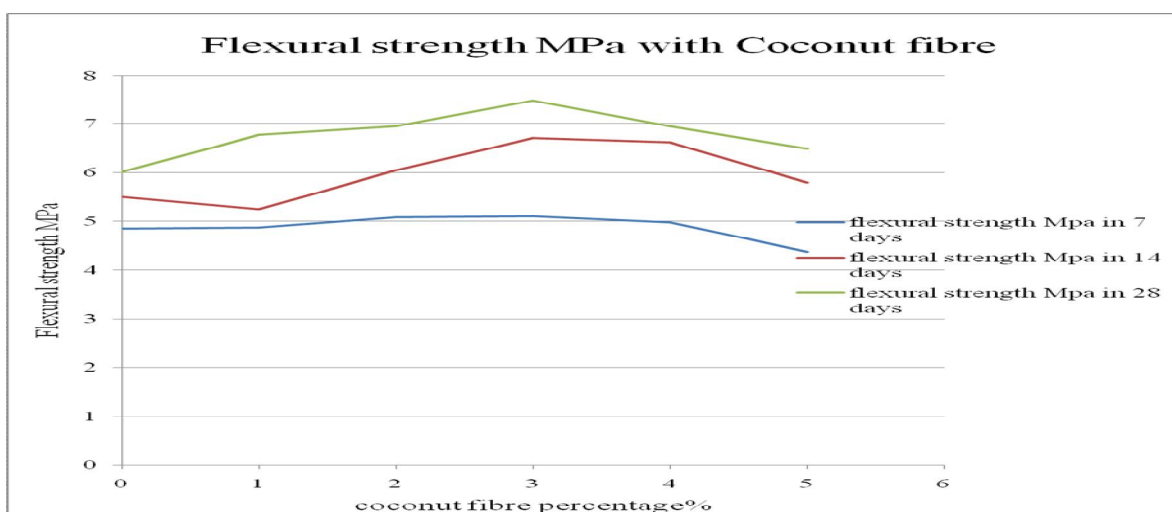
Figure 13: Comparative study on flexural strength (MPa) of concrete with coconut fibre after 7,14 and 28 days curing
