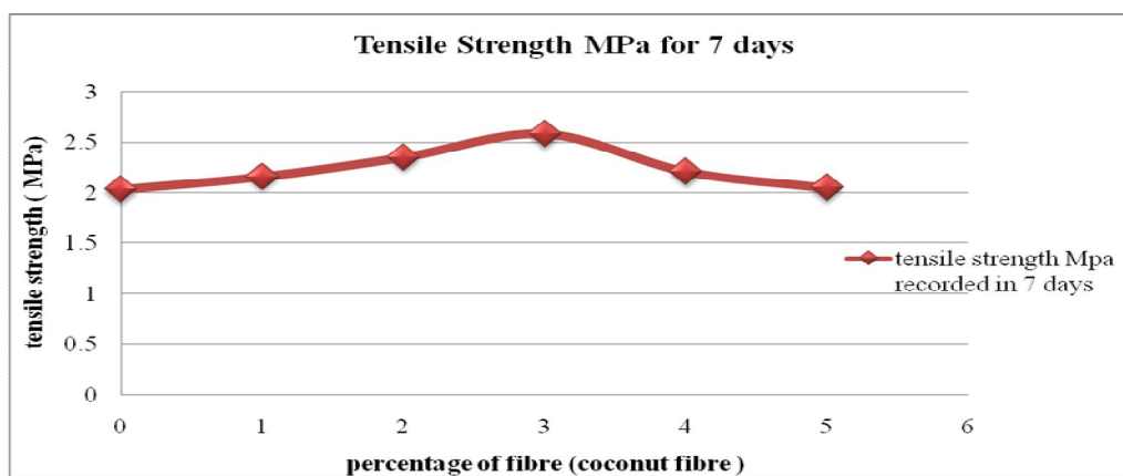
Fig 6: Tensile strength of concrete with coconut fibre reinforcement after 7 days of curing
