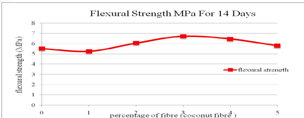
Figure 11: Flexural strength (MPa) of concrete with coconut fibre after 14 days of curing
