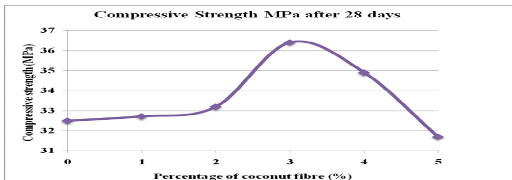
Fig 4: Compressive strength of coconut fibre reinforced concrete after 28 days of curing
