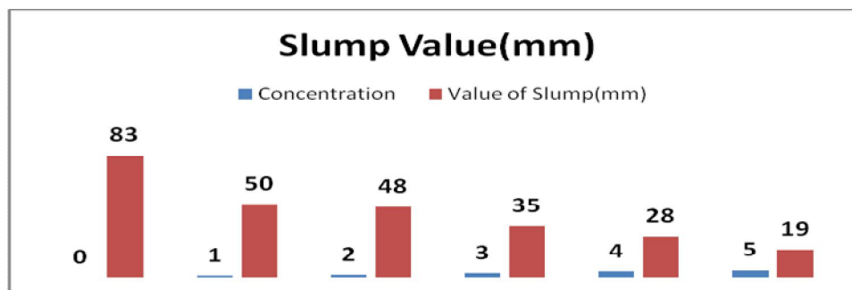
Fig 1 : Slump values for different percentages of coconut fibre in a concrete mix.
