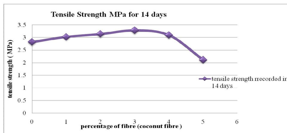
Fig 7: Tensile strength of concrete with coconut fibre reinforcement after 14 days of curing
