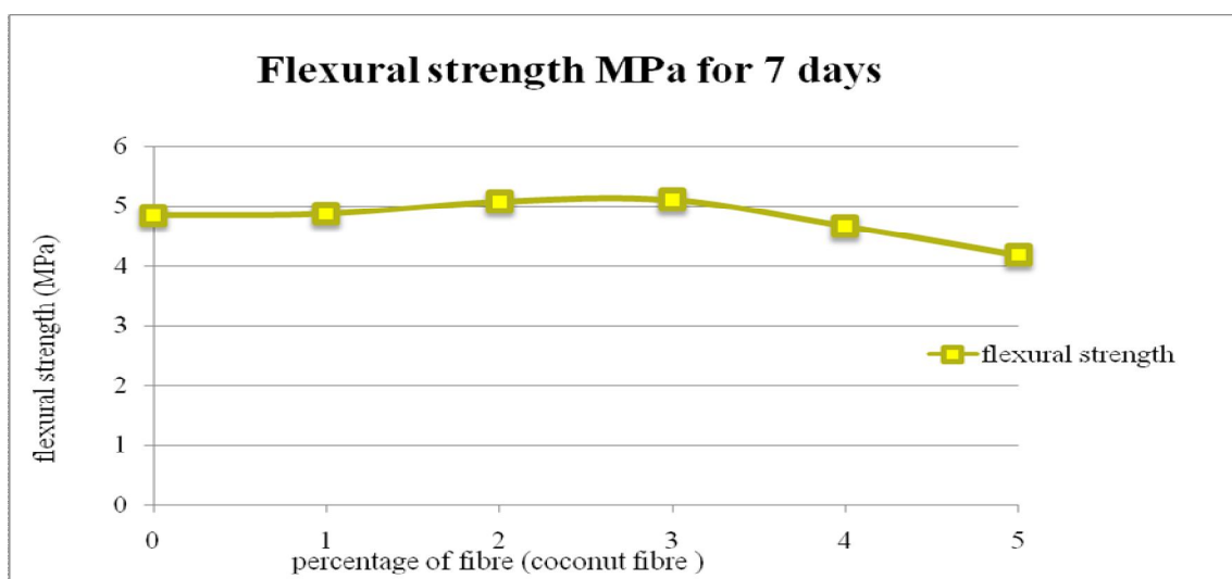
Figure 10: Flexural strength (MPa) of concrete with coconut fibre after 7 days of curing
