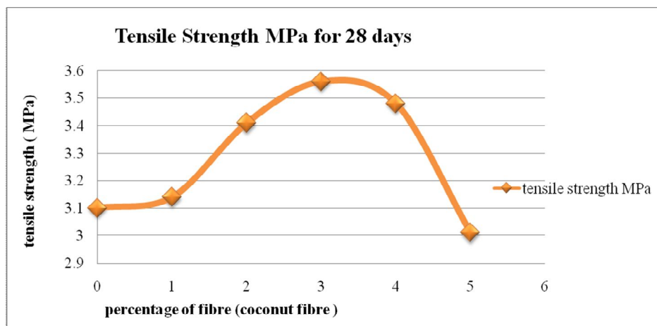
Fig 8: Tensile strength of concrete with coconut fibre reinforcement after 28 days of curing
