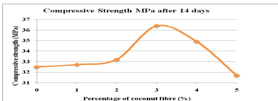
Fig 3: Compressive strength of coconut fibre reinforced concrete after 14 days of curing
