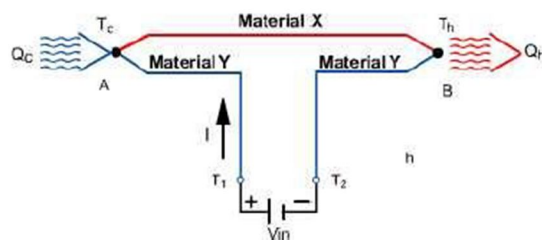
Fig. 1.1. Peltier Effect [10]
