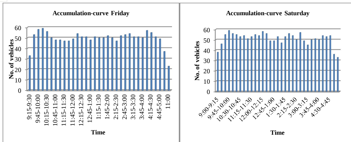
Figure 5: Vehicle accumulation graph of P4 on Saturday
