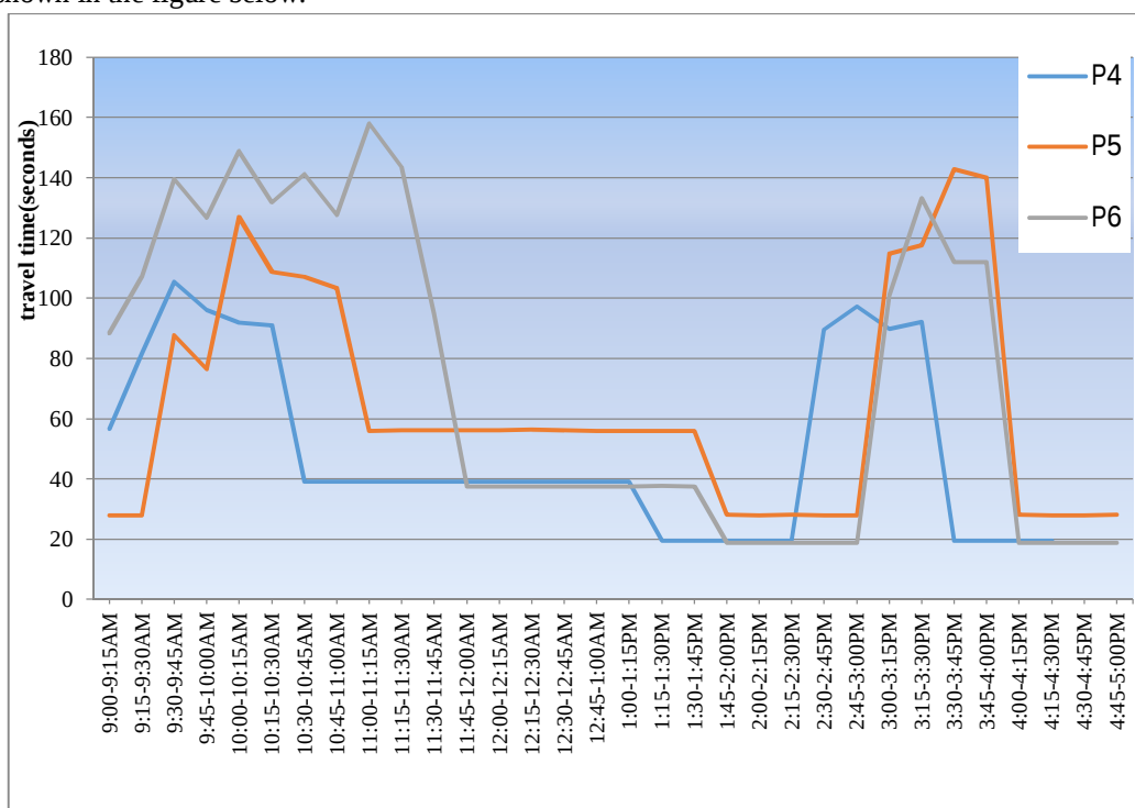
Figure 10 Travel time for roadside parking along the road segment
