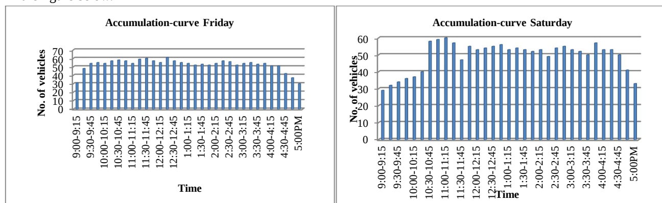
Figure 7: Vehicle accumulation graph of P6 on Friday and Saturday
