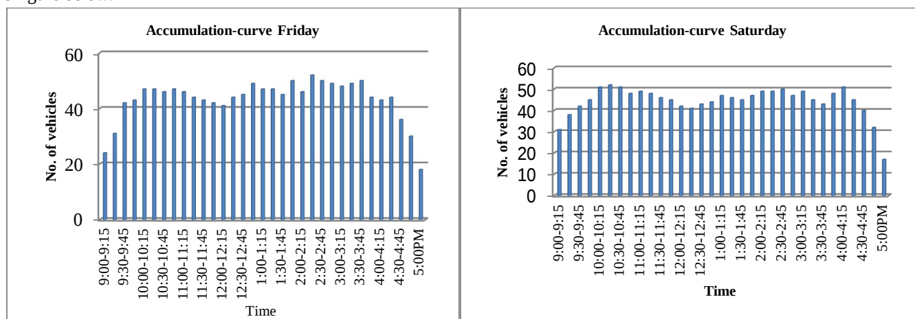
Figure 6 Vehicle accumulation graph of P5 on Friday and Saturday
