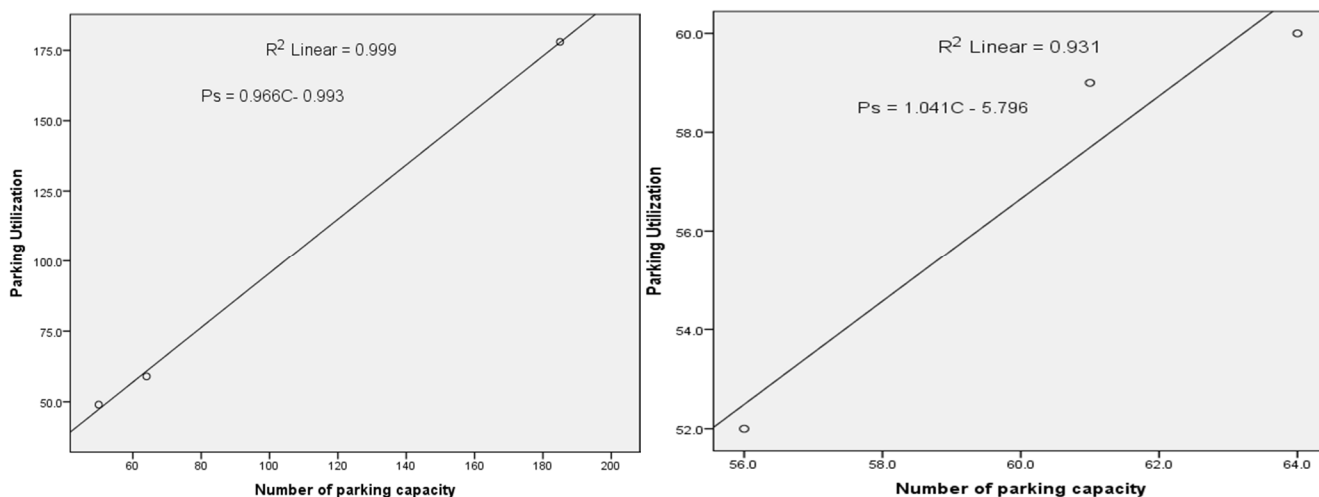
Figure 9 Parking utilized vs. parking capacity graph of off Street and on-street parking
