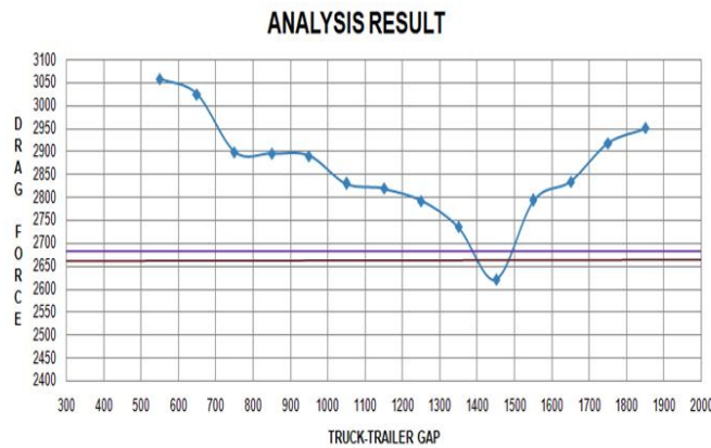
Figure 6: Graph representing the variation of drag force with the increasing gap between truck and trailer
