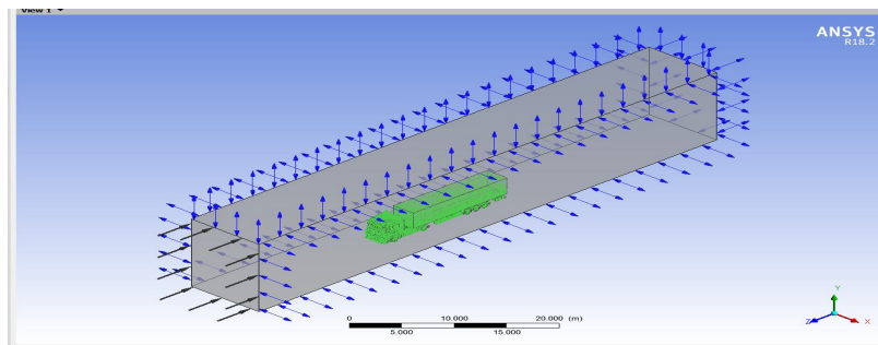
Figure 5: Input boundary conditions
