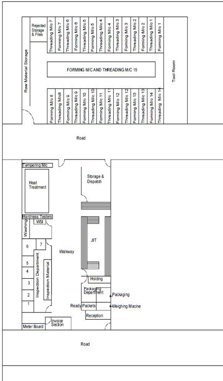
Fig. 6.1 Modified plant layout. [1]
