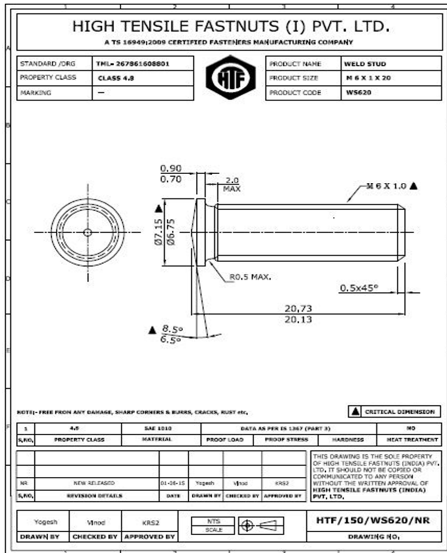
Fig 4.2 Drawing of the job.
