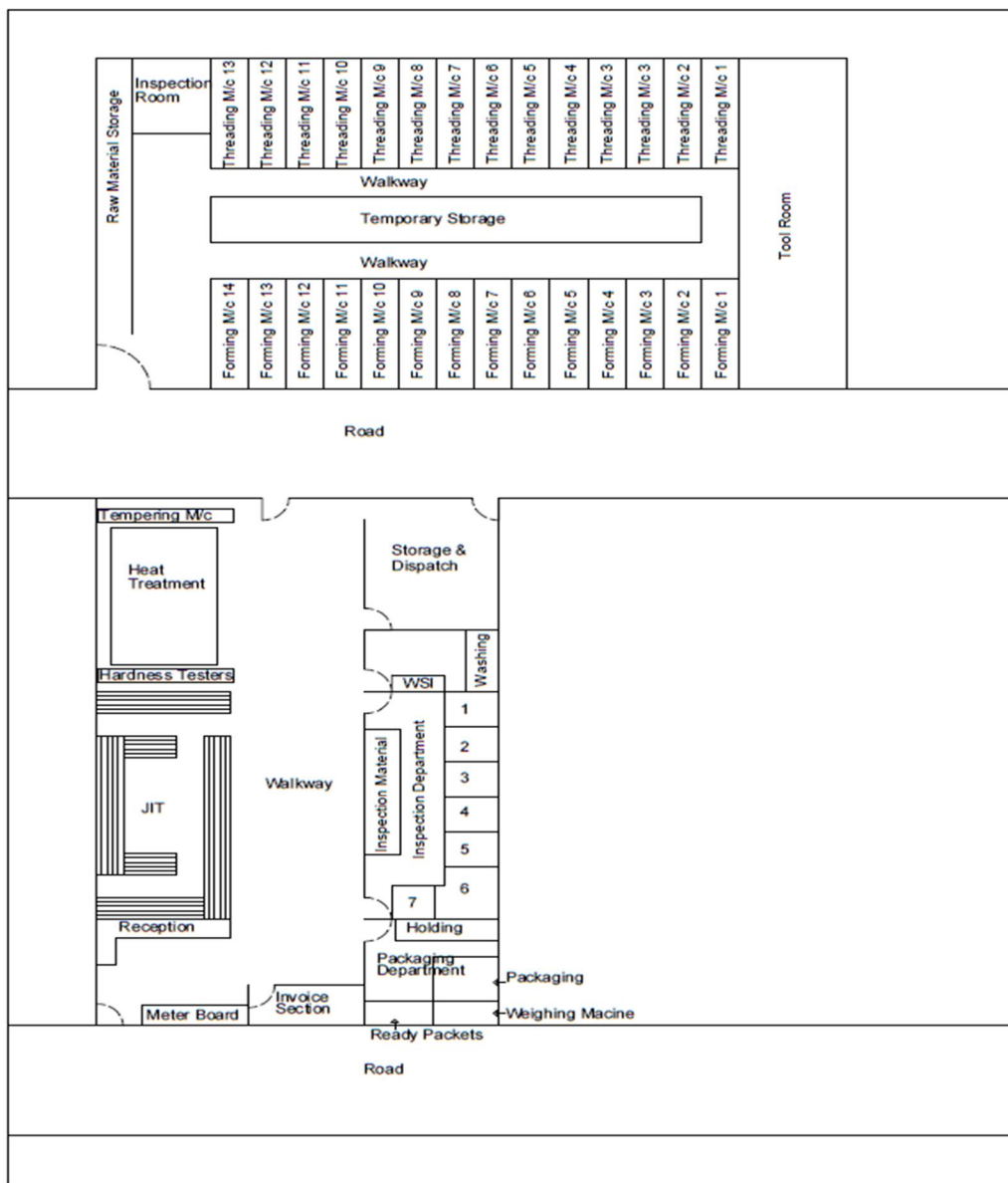
Figure 3.1 Existing plant layout [1]
