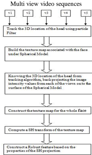
Fig 1: Flow diagram of Multi-view Face Recognition Algorithm
