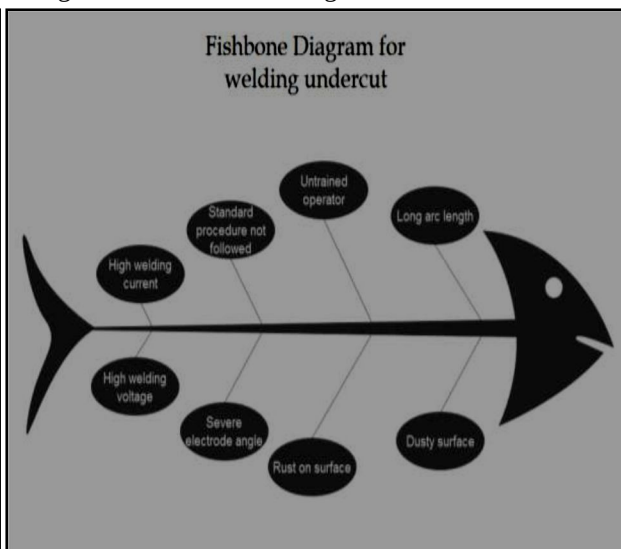
Figure – 11 - Fishbone Diagram for Weld Burn
