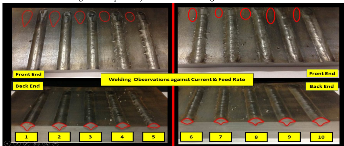
Figure 5 – Ten weld arc observations out of the SMAW trial &amp; error method on MS flat plate
