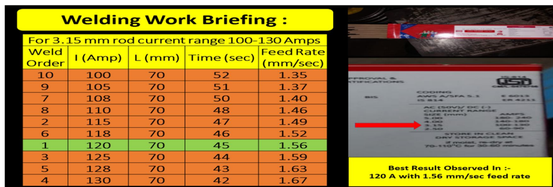
Figure 6 – Calculation of the specific feed rate with respect to set of ten variables of current and respective time duration taken in the welding experimental work
