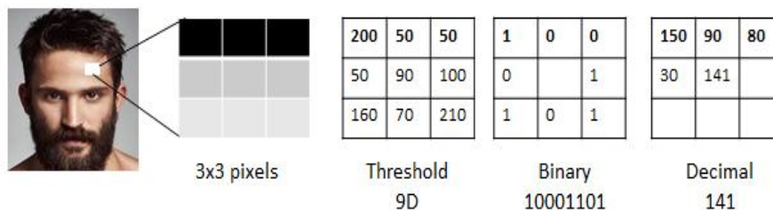
Fig.4. LBP feature extraction steps
