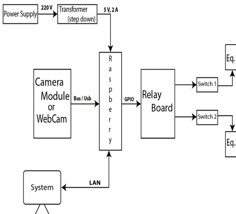
Fig 3. Proposed Methodology for Smart Classroom
