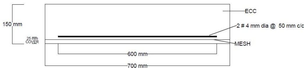
TYPE IV : ECC REINFORCED BEAM WITH MESH
