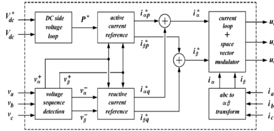
Fig. 2. Diagram of the STATCOM control system.
