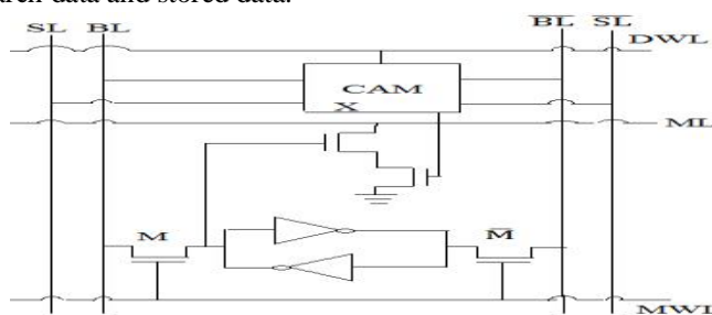
Fig.5 Schematic of a 4T-Ternary CAM cell
