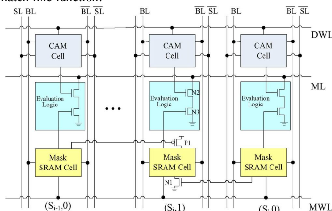
Fig. 3 Two-Side Self-Gating Ternary CAM array
