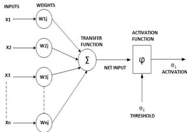
Fig.2 Mathematical Modeling of ANN
