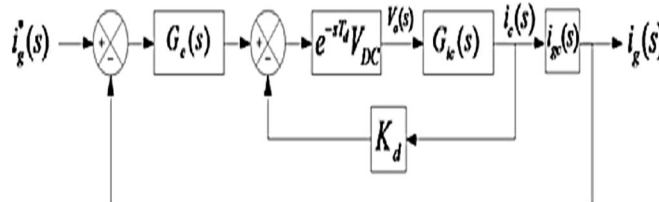
Fig.4 Dual loop regulator with capacitor current active damping.
