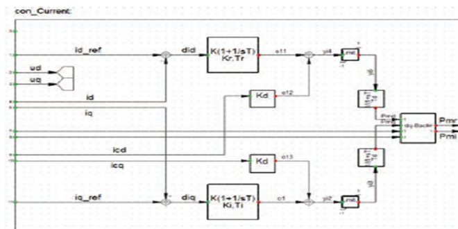
Fig 9 current control block
