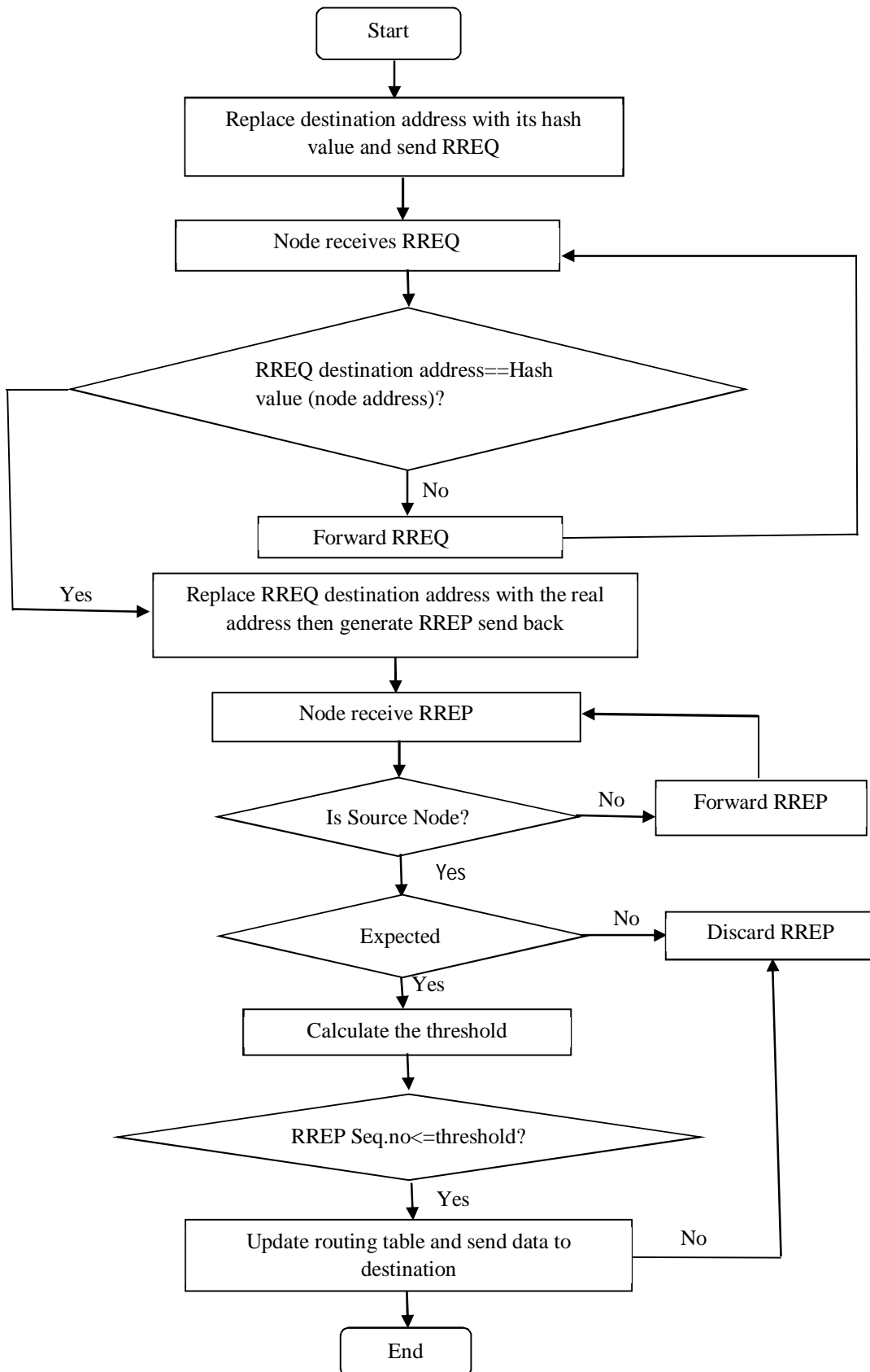
Figure 2: Flow graph of proposed work
