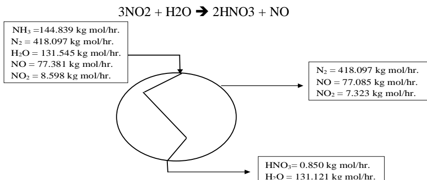
Figure 4: Material Balance on Cooler and Condenser
