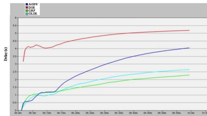
Figure 6. Delay (s) comparison in four routing protocols
