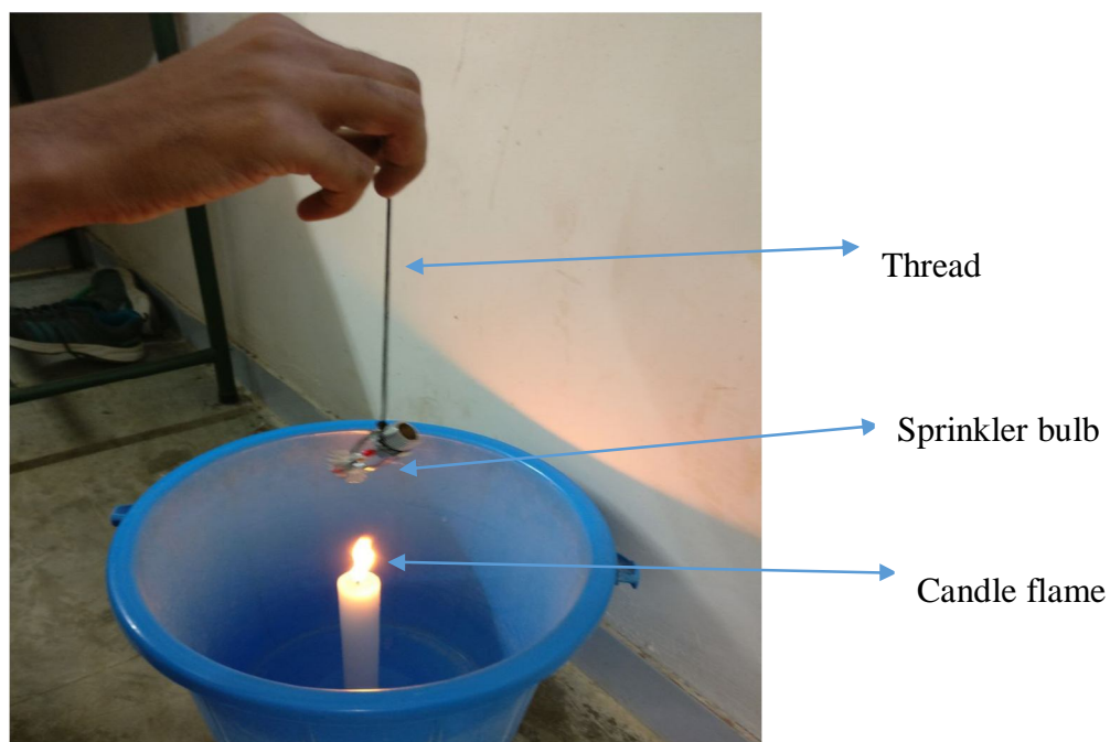
Fig 4.20 Experimental setup
