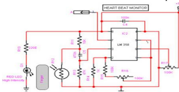
Fig 2: - Heart Rate Sensor Circuit Diagram
