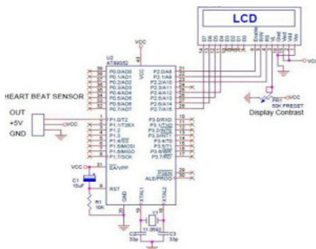
Fig 3: - Control Unit Diagram
