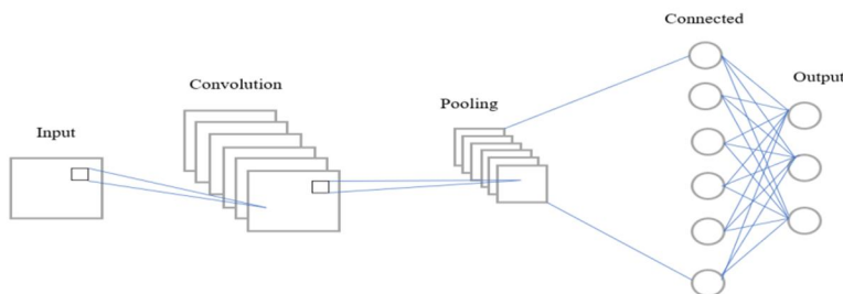
Figure 3. CNN Architecture
