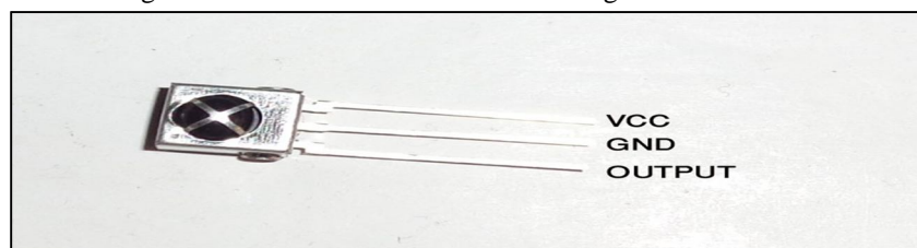
Figure 1 IR Sensor
