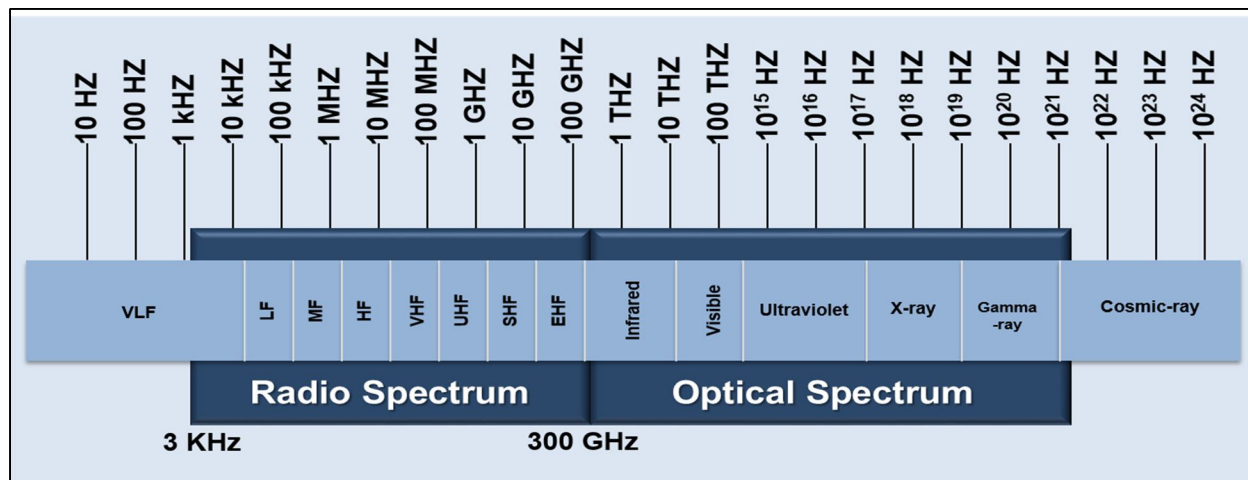
Figure 6 Electromagnetic Spectrum
