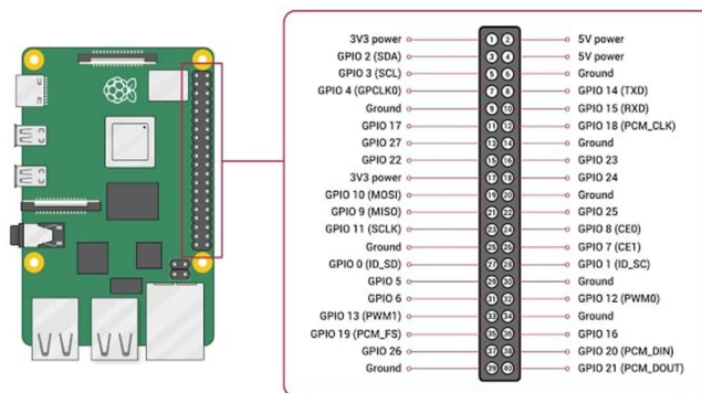
Fig 3: Pin Configuration Of Raspberry-Poi Board
