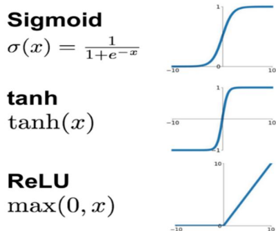
Figure 3. Activation functions
