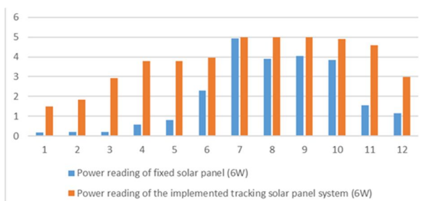
Figure 4: Graph of power readings for a cloudy morning and sunny afternoon, 11 th March, 2017.
