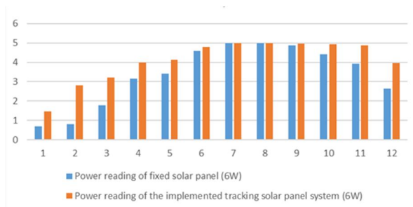
Figure 5: Graph of power readings for a bright sunny day, 12 th March, 2017.
