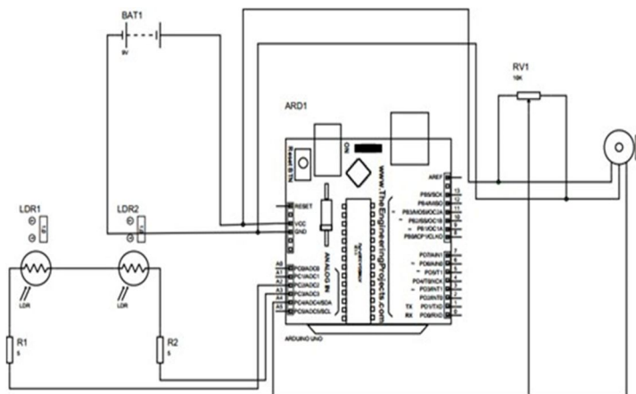
Figure 3: Schematic diagram of the solar panel tracking system.
