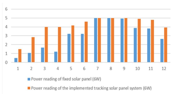
Figure 6: Graph of power readings for a bright sunny day, 13 th March, 2017.
