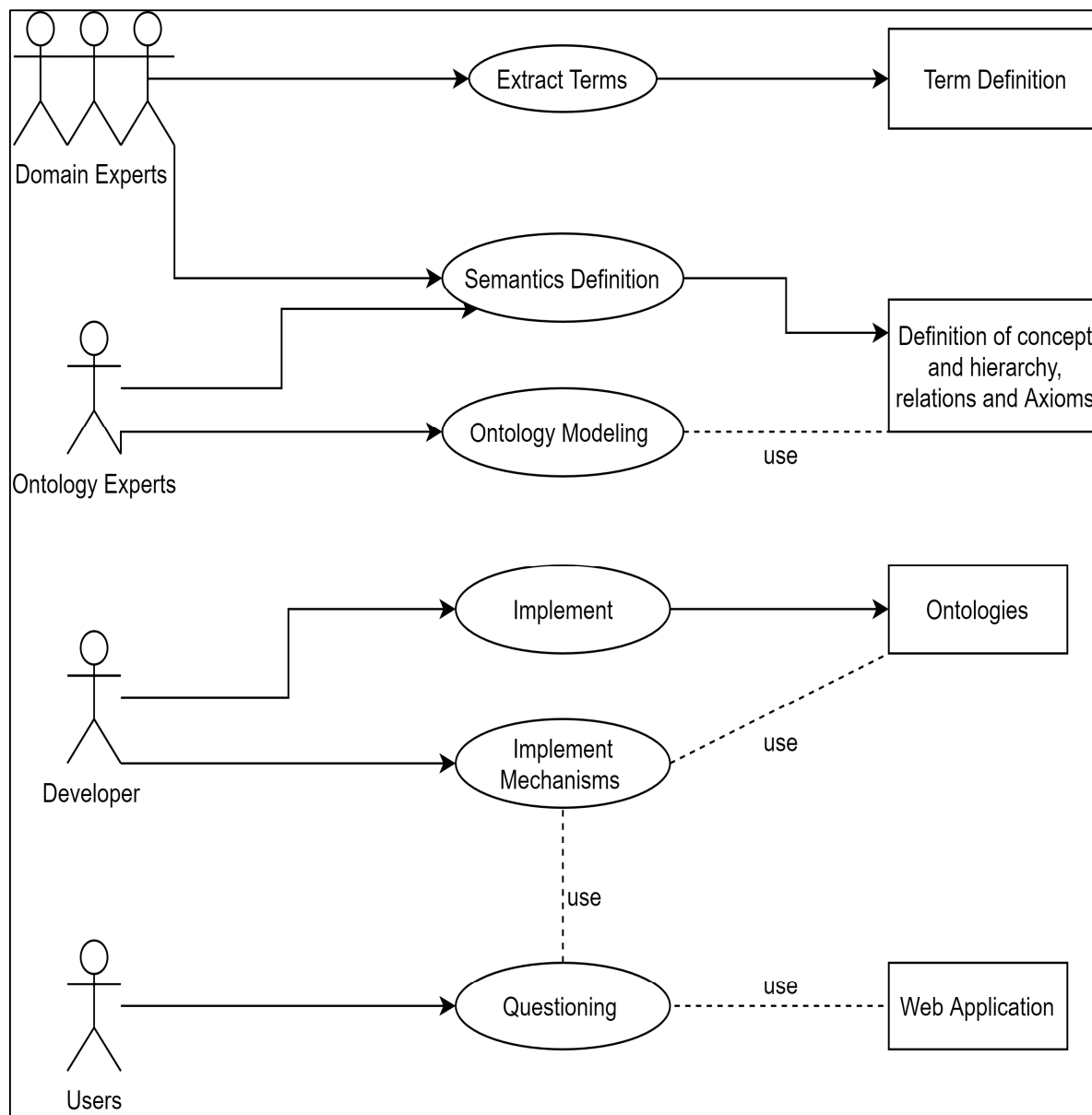
Figure 1. Ontology Development Methodology
