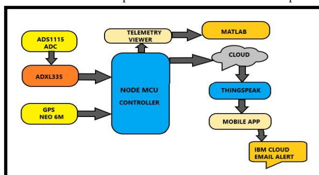
Fig.2.System'sBlock diagram
