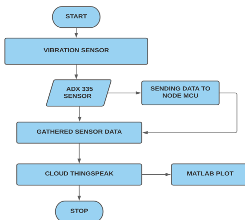
Fig.1.System'sflowchart
