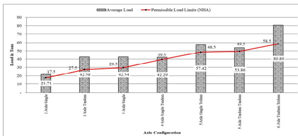
Fig. 10 Gross Vehicle Weight vs Permissible Load Limit
