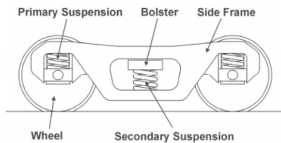
Fig.1 Typical bogie components (Steffens 2005)
