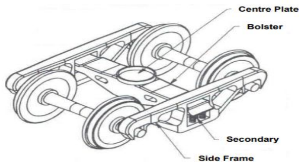
Fig.2 Three piece bogie (Steffens 2005)
