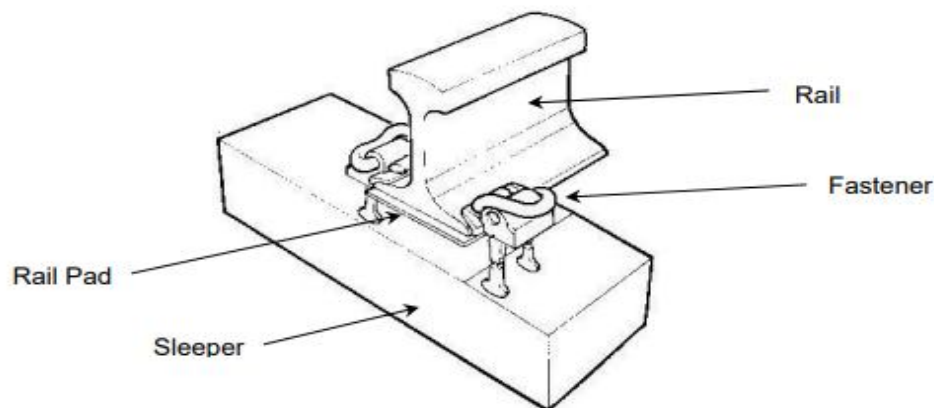
Fig.4 Concrete sleeper fastening system (Steffen 2005)
