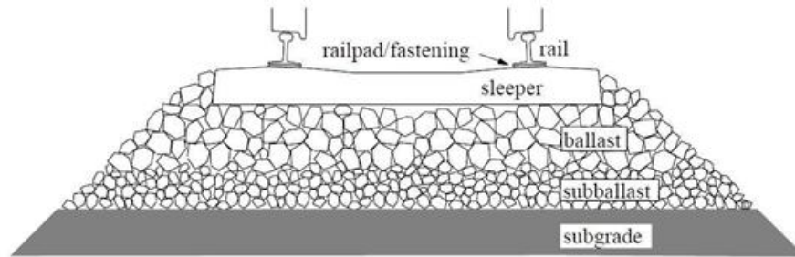
Fig.3 Track with different components (Steffens 2005)
