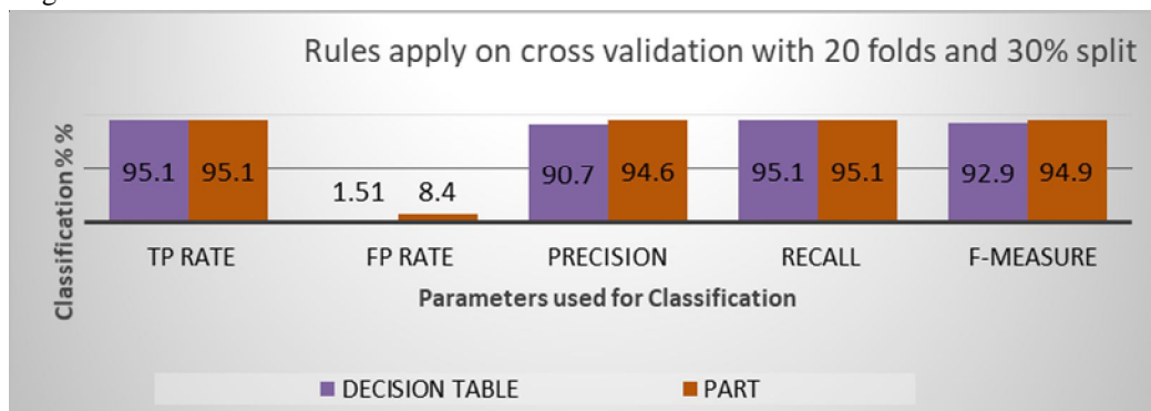
Fig.6: Rule based classifier applied on cross validation with 20 folds and 30% split data
