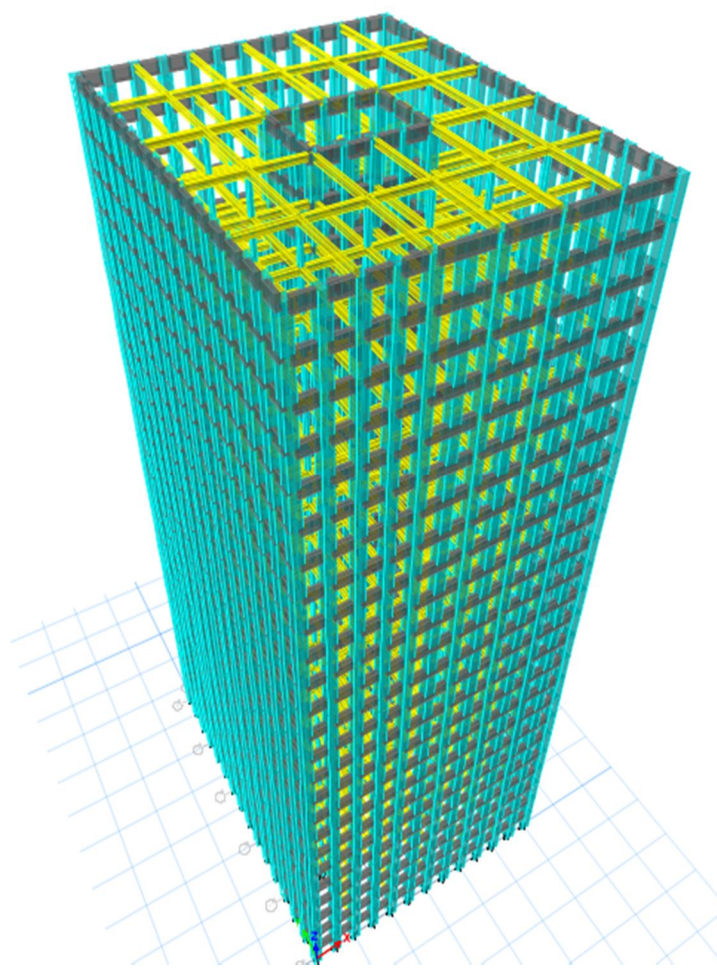
Figure 1:3D view of tube in tube structure
