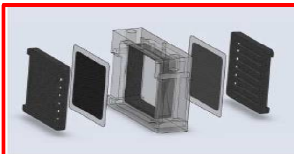
Fig.(12) Single Cell Bio battery
