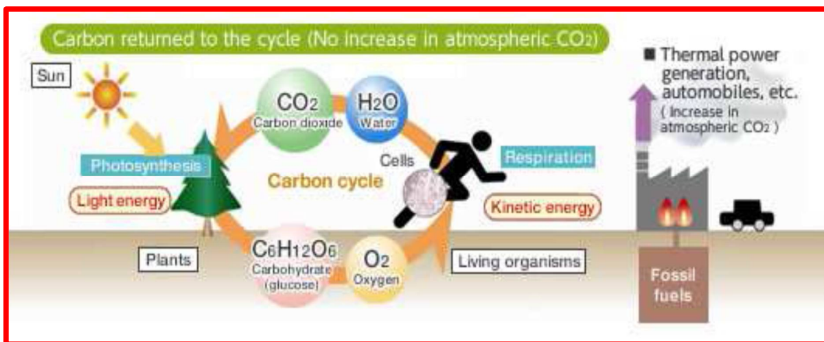
Fig.(2) Carbon cycle
