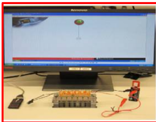
Fig.(15) Sensor and Wireless Transmitter running on a bio-battery
