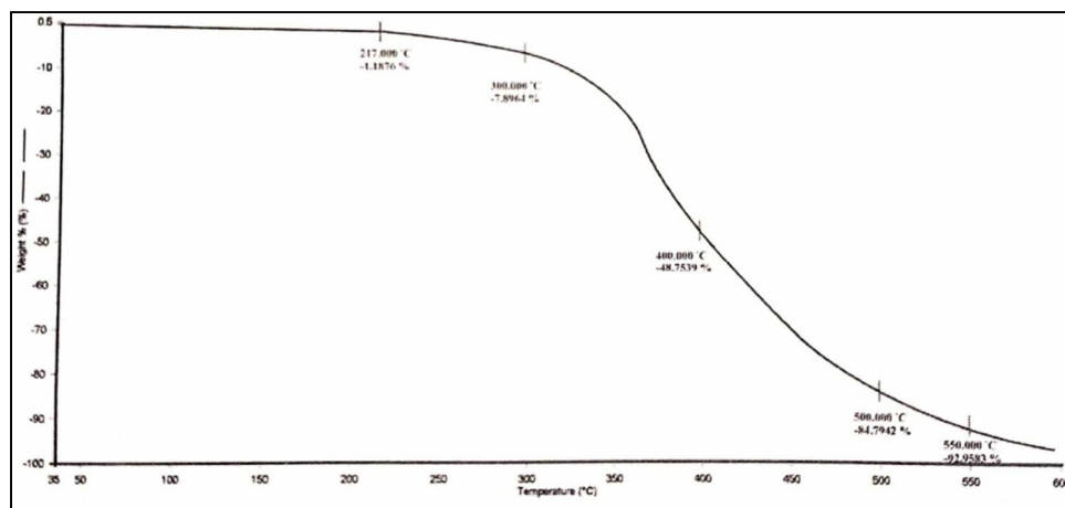
Fig. 14. Thermograms for PNPMCAN
