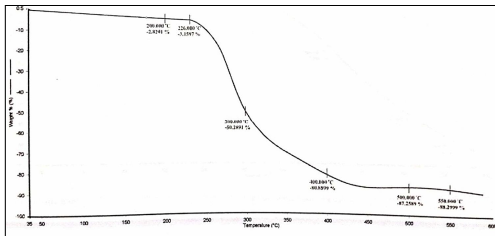
Fig.13 Thermograms for PNPMCAN
