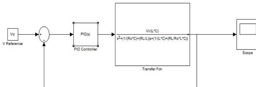
Fig.3 Transfer function model with PID Controller
