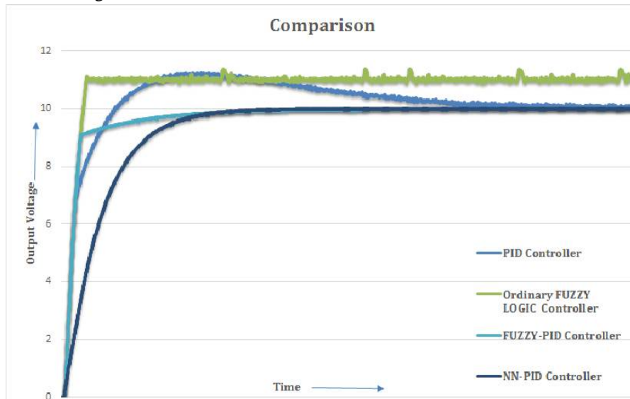
Fig.11 Comparison of Output Voltage Waveform of Various Controllers
