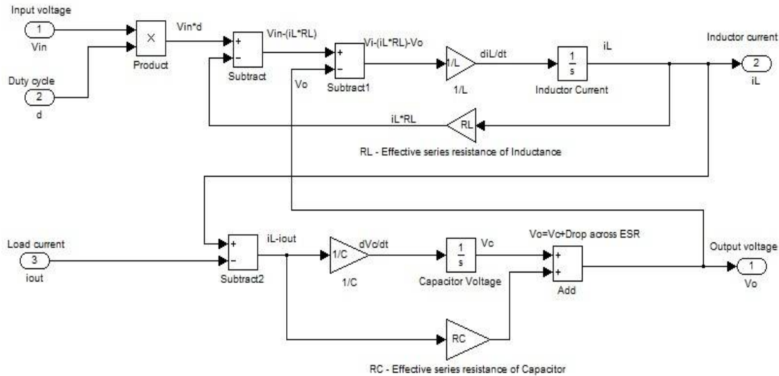
Fig.1 Subsystem for Buck Converter
