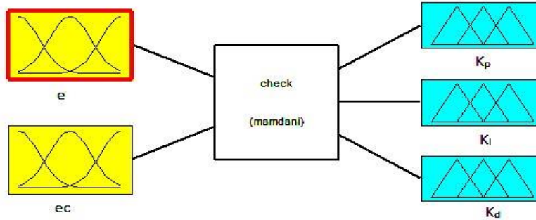
Fig.4 Two Input-Three Output Fuzzy Logic Controller Structure
