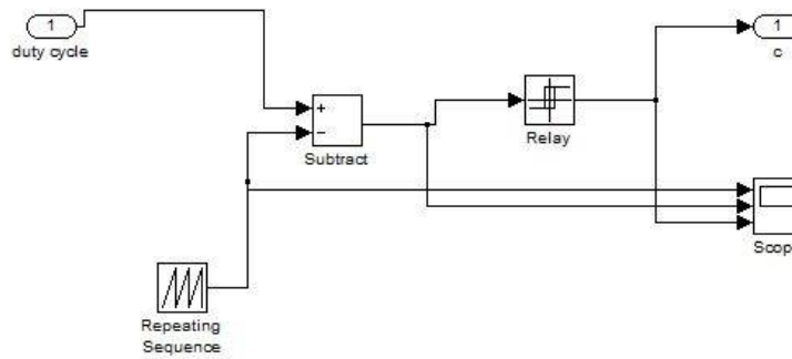
Fig.2 Subsystem for PWM Waveform Generator
