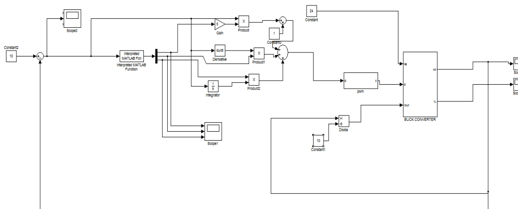
Fig.9 Simulated Model of NN-PID Controller for Controlling Buck Converter
