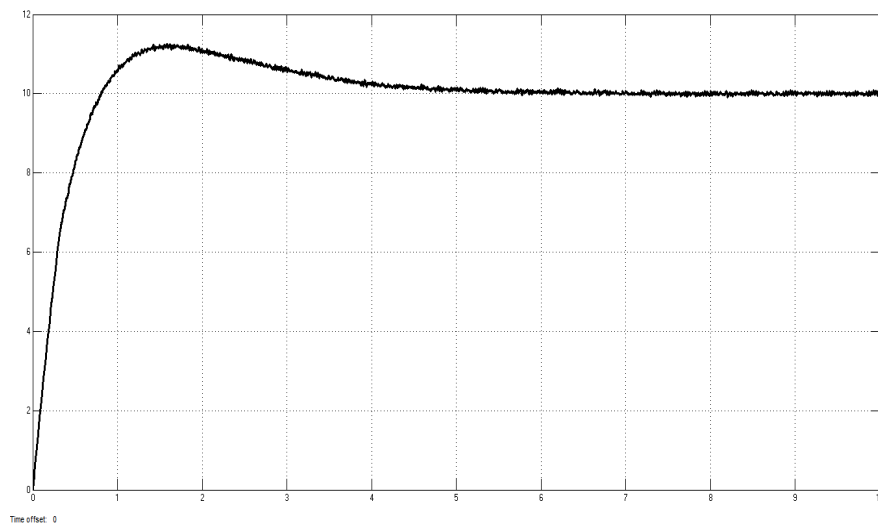
Fig.6 Output Voltage Waveform of PID Controller
