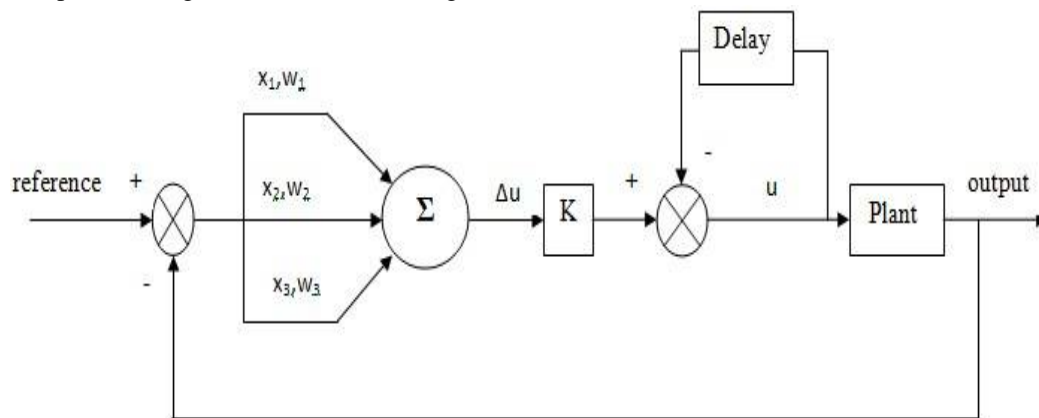
Fig.5 Single Neuron ANN Structure
