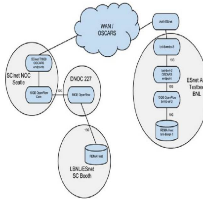
Figure 1: Network architecture for SC11 ECSEL demonstrator
