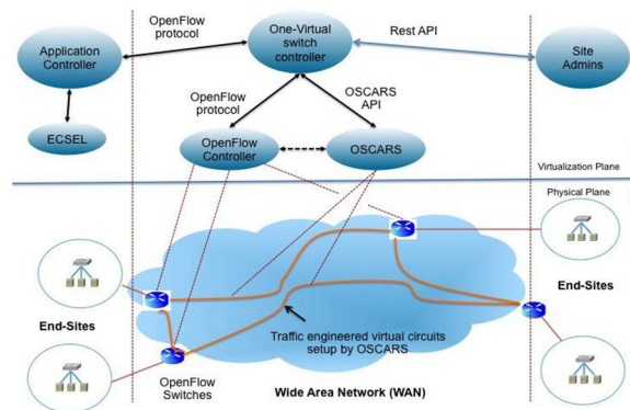
Figure 3: End-to-end virtualization using One-Virtual-Switch, ECSEL and OSCARS
