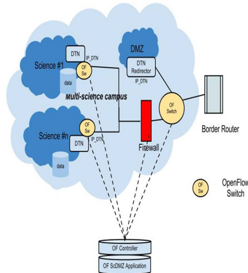
Figure 2: OpenFlow-based end-site architecture to support multiple science disciplines
