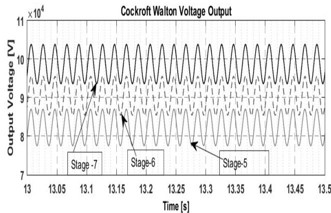
Figure 9 Ripple Voltage Level of Output Stages
