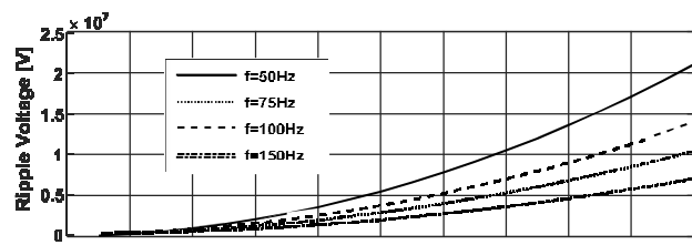
Figure 4 Ripple Voltage in CWVM as different Frequency Level
