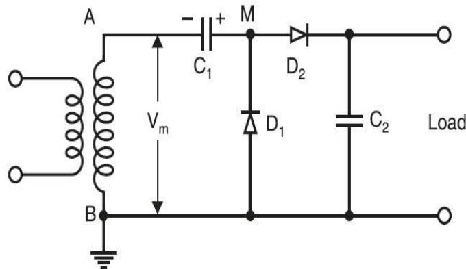
Figure 1 Grienacher Voltage Doubler Circuit
