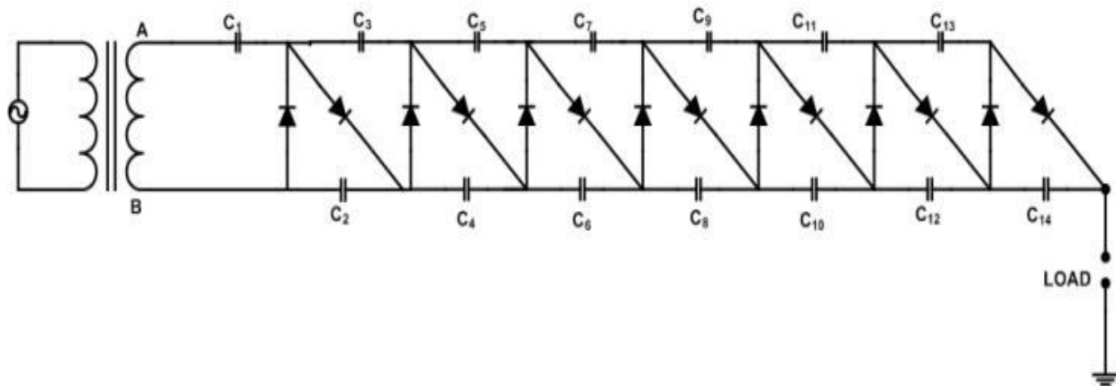
Figure 2 Seven Stage CWVM Circuit
