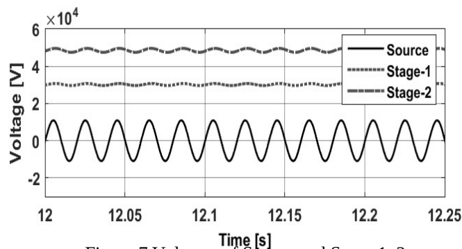
Figure 7 Voltages of Source and Stage-1, 2
