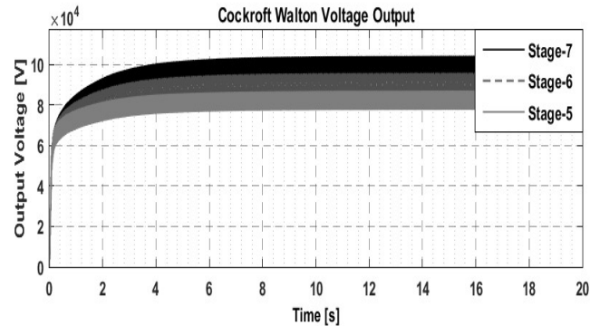
Figure 8 Output of Final Three Stages
