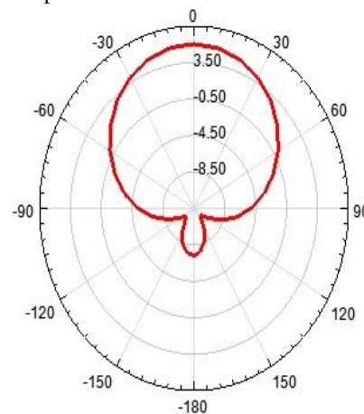
Figure 7 Elevation pattern (E-Plane) gain display (for \theta =all values and \phi = 0 degree)
