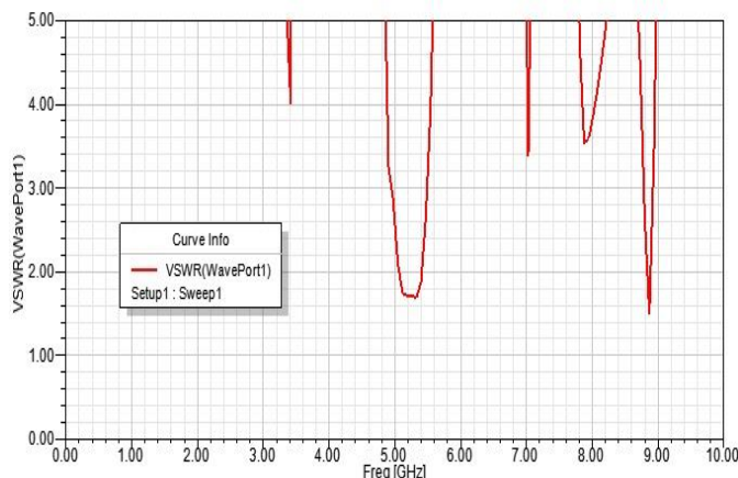
Figure 10 VSWR plot for the dual band array antenna
