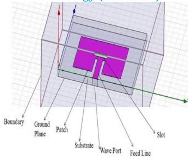
Figure 2 Simulated geometry of dual band antenna design
