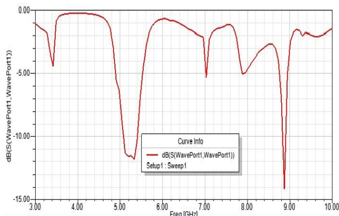
Figure 9 Return loss graph for dual band array antenna
