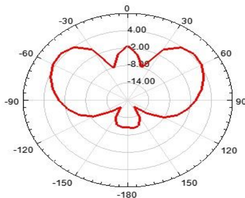
Figure 11 Elevation pattern (E-Plane) gain display (for \theta =all values and \phi = 0 degree)
