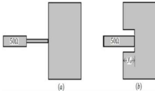
Figure 1 microstrip patch antenna with feed form side
