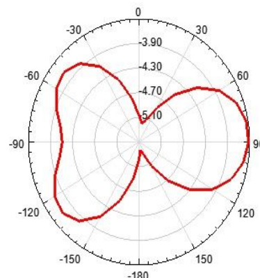
Figure 8 Azimuthal pattern (H-plane) gain display (for \phi = all values and \theta = 90 degree)
