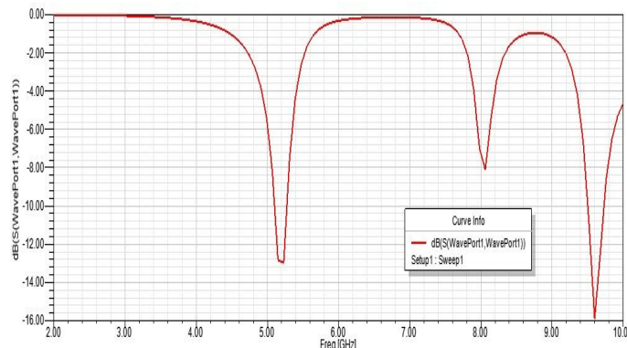
Figure 5 Return loss graph for dual band antenna
