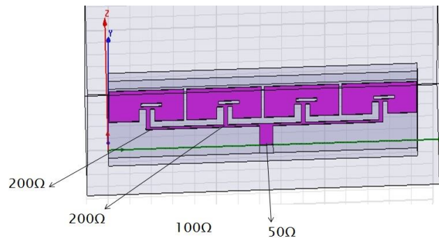
Figure 4 Simulated dual band array antenna design
