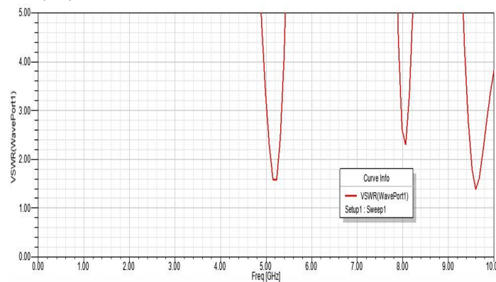
Figure 6 VSWR plot for the dual band antenna
