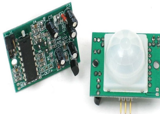
Fig3: PIR Sensor
