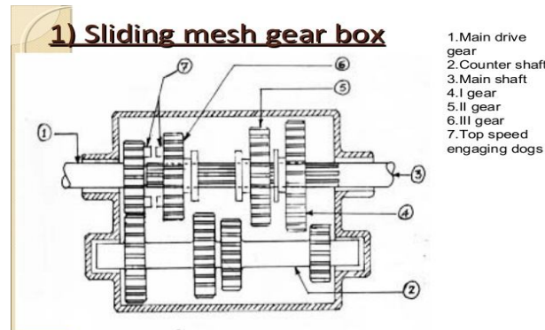
Fig. 4.3 Type of Gear Box
