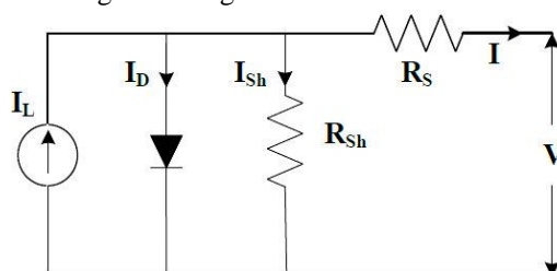
Figure 2: Photo-Voltaic model
